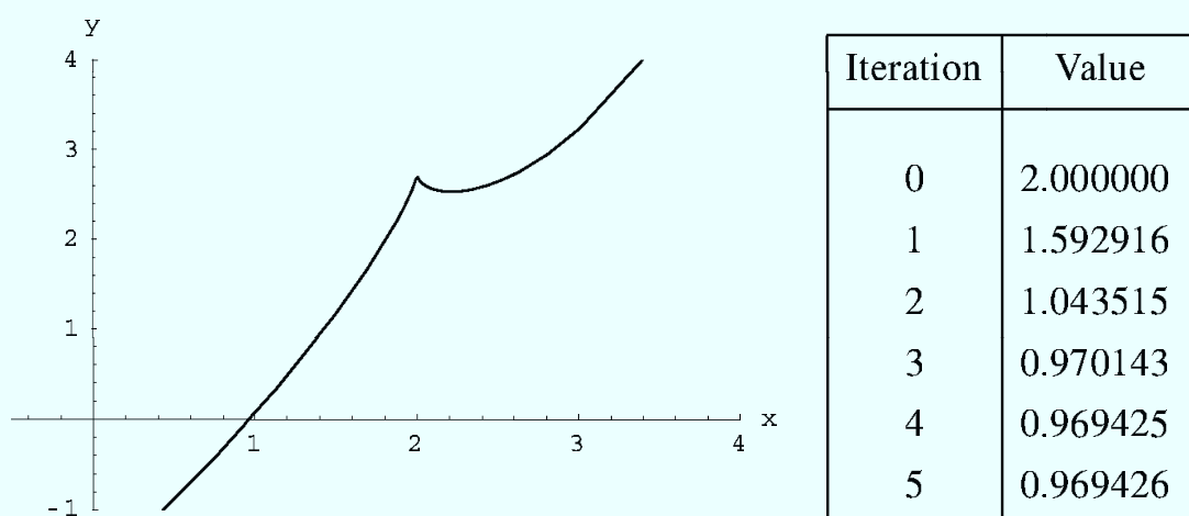
Figure 1. The function is not differentiable in the initial point, but it does not have influence to convergence.
