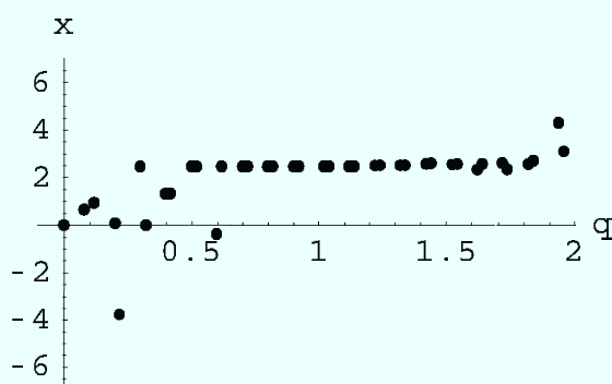
Figure 2. Solving of the equation with multiple roots. The values of the iterations from n = 100 to n = 140 .
