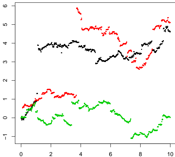
3 trajectories of a stable process
