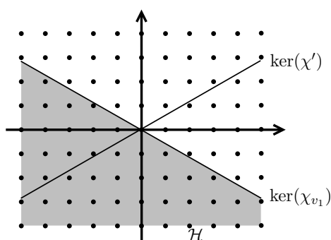
FIGURE 1. The halfspace \mathcal{H} is bounded by the kernel of a Lyapunov weight. The kernel of the non-proportional weights is also shown.
