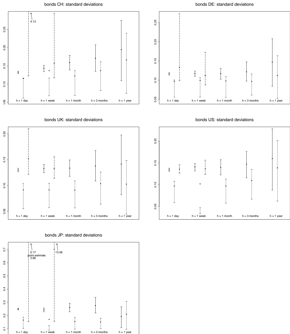
Figure 3 10-year government bonds: estimates for standard deviations (including confidence intervals constructed via simulation), using random walk models (full lines), AR( p ) models (dotted lines) and GARCH(1,1) models (dashed lines).
