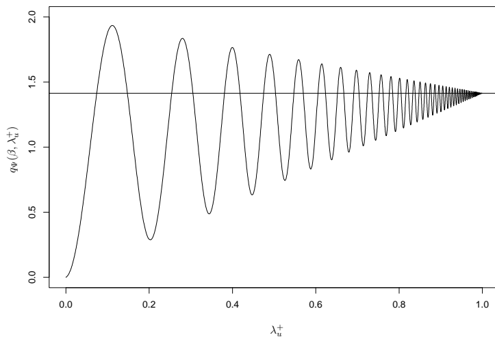
Figure 4: q_{\Psi}(\beta, \lambda_u^+) as a function of \lambda_u^+ for the Fréchet family copula (6.1) with parameters p_1 and p_2 from (6.3) and (6.4), respectively. Subadditivity occurs below the horizontal line, superadditivity above.
