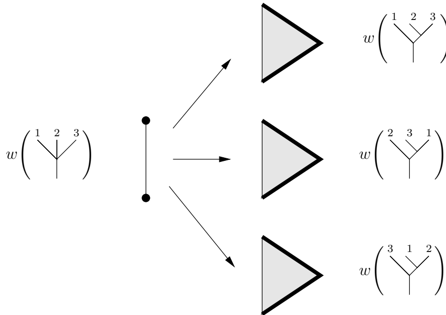
Figure 4: Spaces of weightings of trees with three leaves
