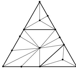
Figure 15: The subdivision of a face \sigma
