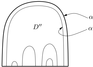
Figure 10: The disk D , showing D \cap H and D''
