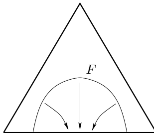
Figure 3: A weight-reducing isotopy
