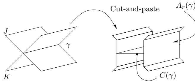
Figure 5: The exchange band for \gamma
