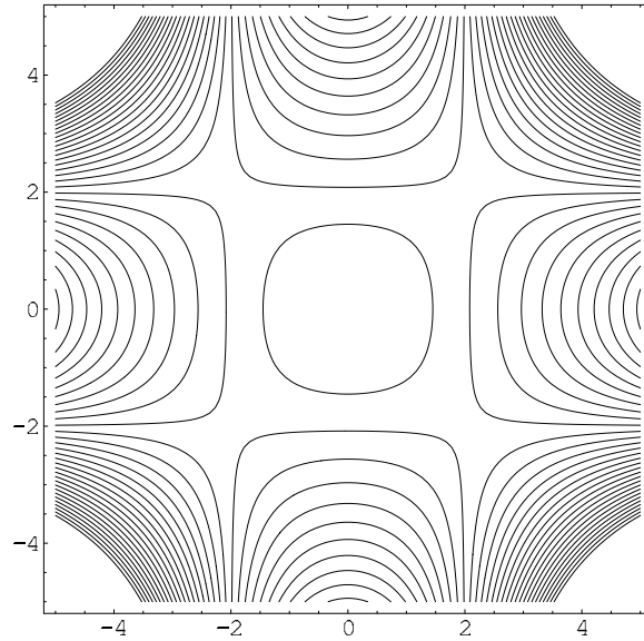
Figure 9: Level sets of (x^2 - 4)(y^2 - 4)
