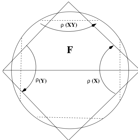
Figure 10: Fundamental hexagons for a hyperbolic three-holed sphere
