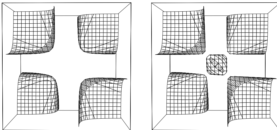
(a) Level set \kappa = -2.1
