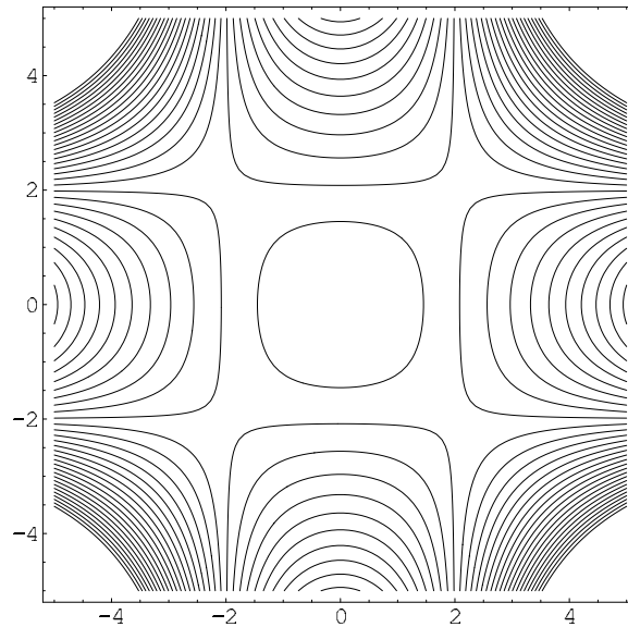
Figure 9: Level sets of (x^2 - 4)(y^2 - 4)
