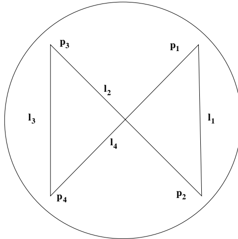
Figure 7: When \overline{p_2p_3} meets \overline{p_4p_1}
