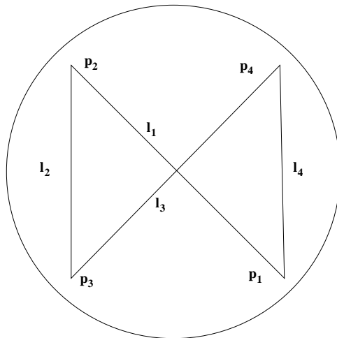
Figure 6: When \overline{p_3p_4} meets \overline{p_1p_2}
