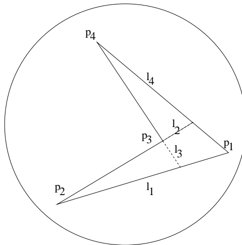
Figure 8: A nonconvex embedded quadrilateral
