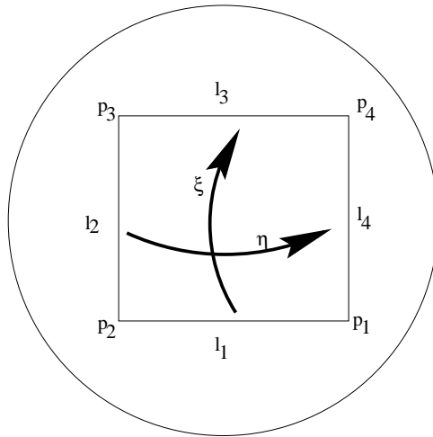
Figure 5: A convex embedded quadrilateral
