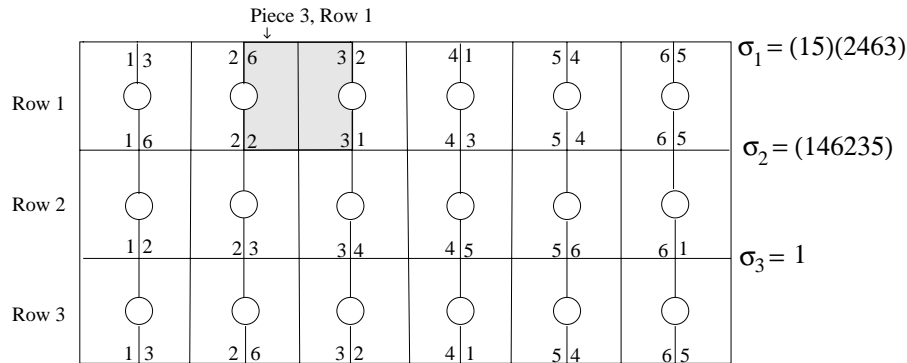
Figure 6: The permutations encode the combinatorics of the gluing
