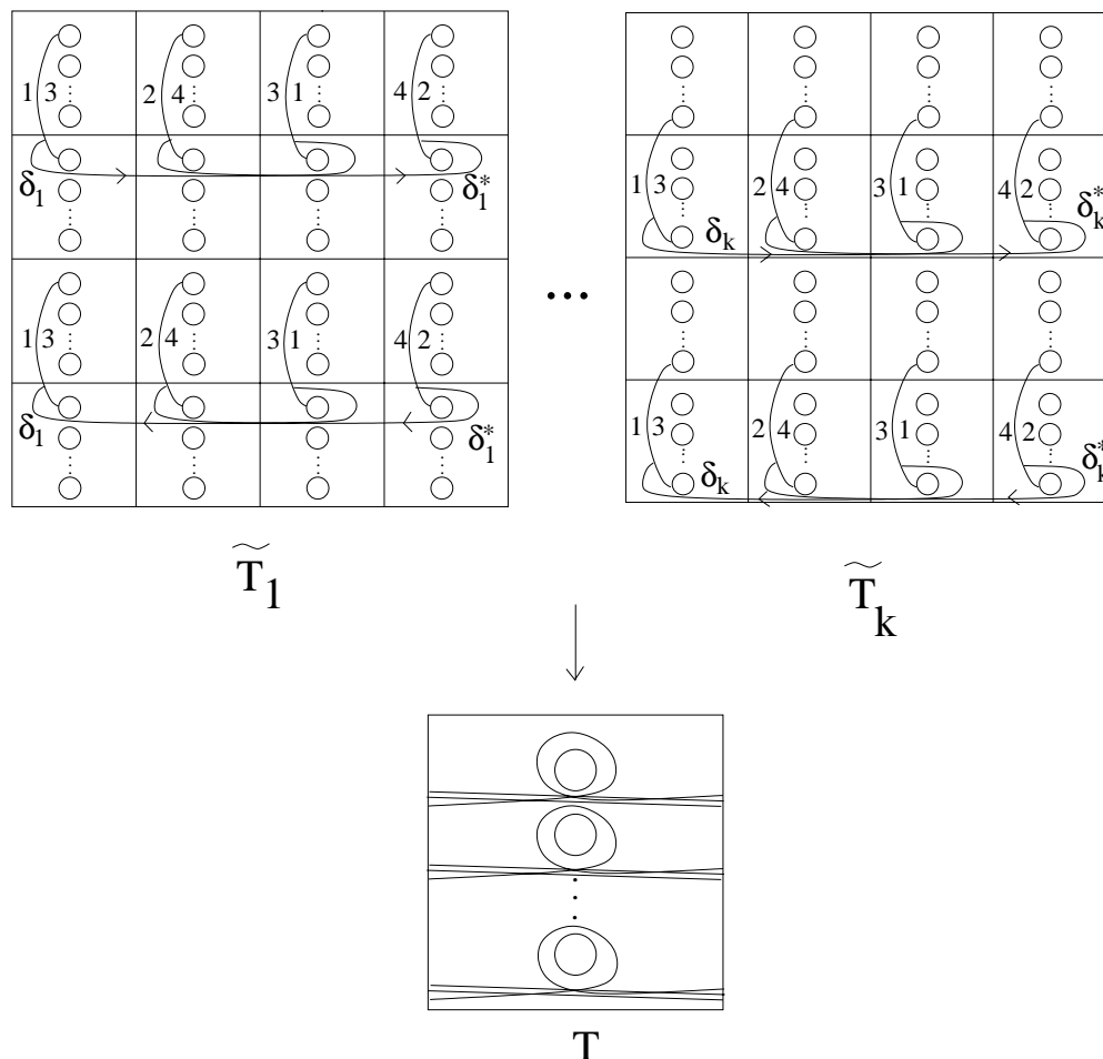
Figure 4: Each boundary component of T gives rise to a different cover.
