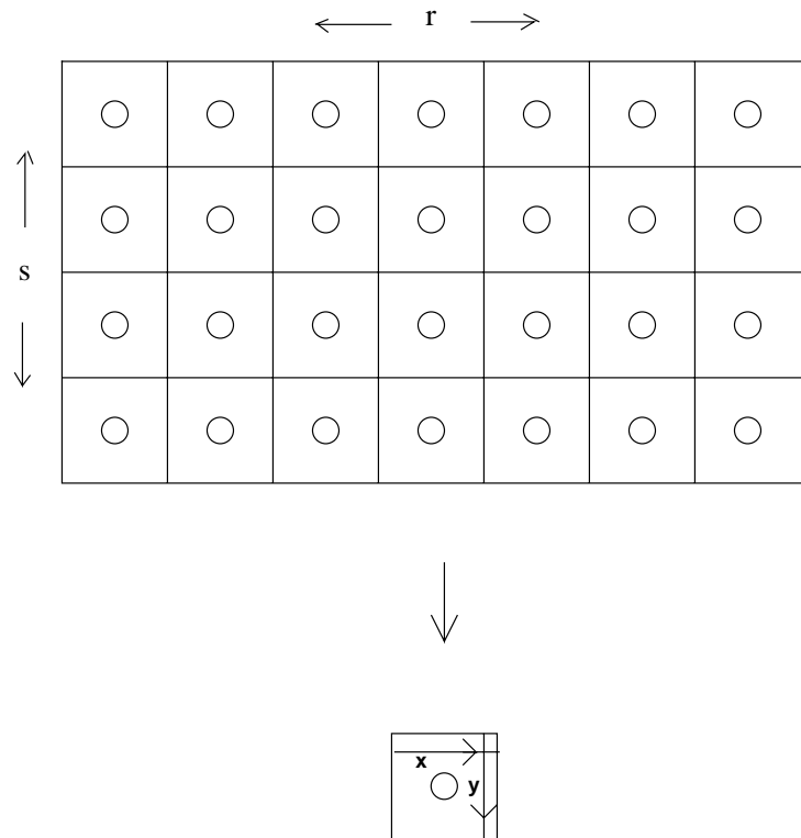
Figure 5: The cover \hat{T} of T
