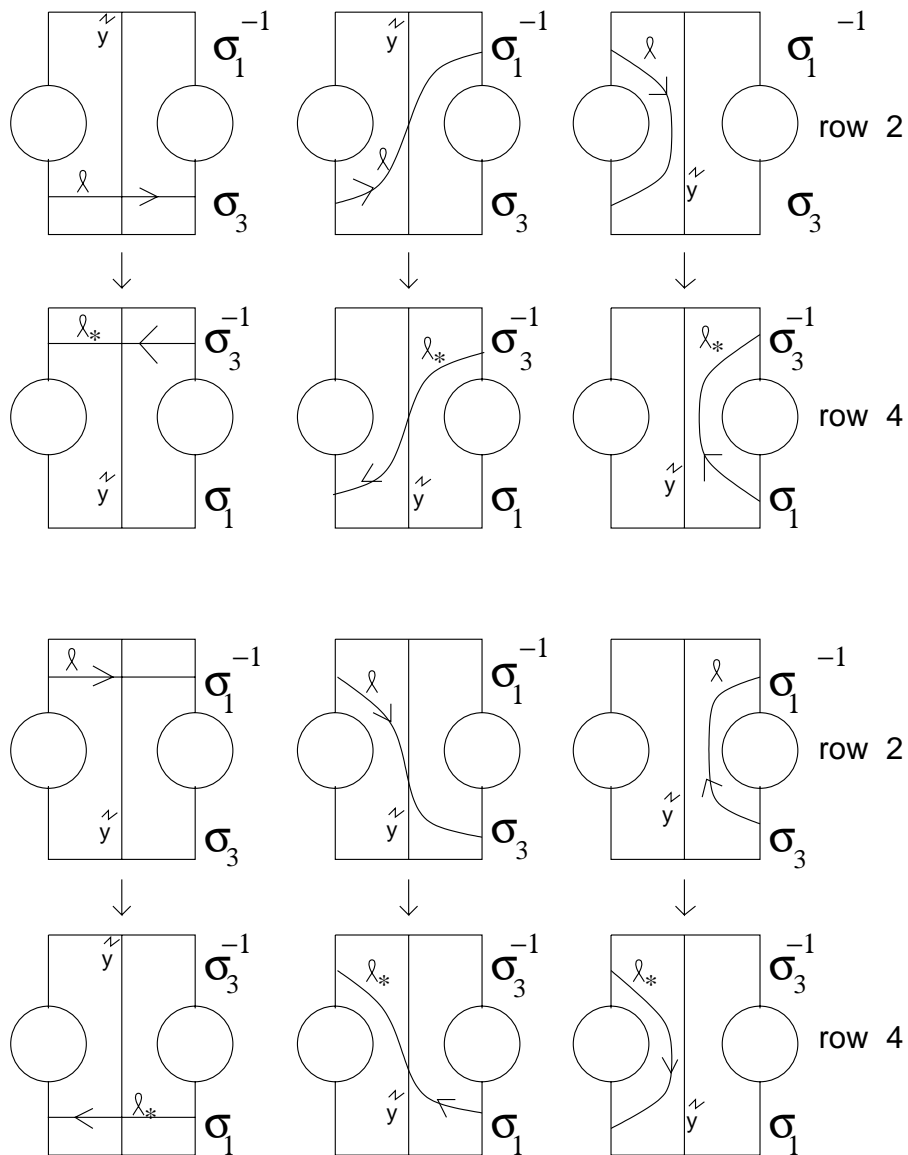
Figure 7: Corresponding to each segment of l , we construct a corresponding segment of l_* .
