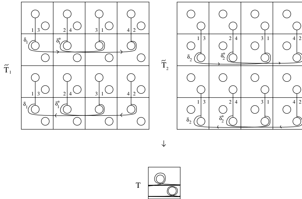
Figure 3: We may arrange for \delta_1 \cup \delta_1^* and \delta_2 \cup \delta_2^* to have disjoint projections.
