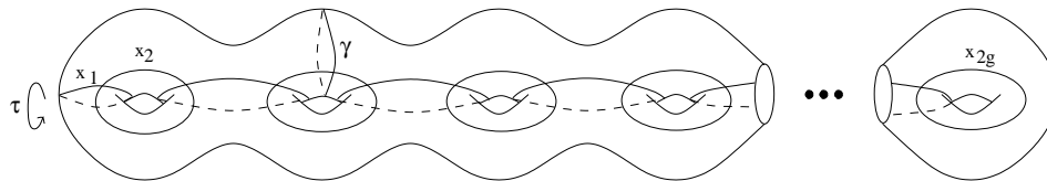
Figure 1: The mapping class group is generated by Dehn twists in these loops.
