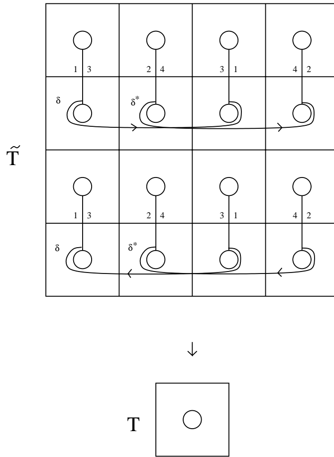
Figure 2: The cover \tilde{T} of T
