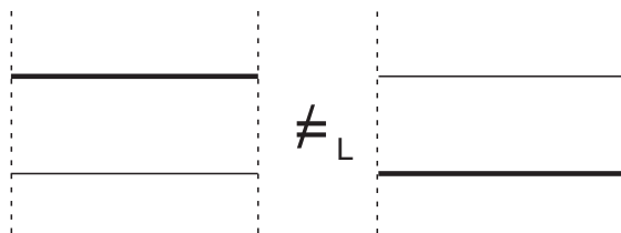
Figure 1.1: The legendrian link (0) and its nonequivalent swap
