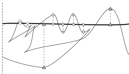
Figure 6.1.1: The legendrian link (2, 2, 4, 1, 2) positioned so that it has a difference function \Delta with (2 + 4 + 2) critical points which are represented as pairs of points ((q_0, p_0, z_1), (q_0, p_0, z_0)) \in \Lambda_1 \times \Lambda_0 . The shifted indices of these critical points are calculated by Proposition 5.5.
