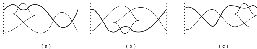
Figure 1.14: The legendrian links (a) (2, 1, 2^0) , (b) (2, 1, 2^1) , and (c) (2, 1, 2^2) . The link (2, 1, 1^0) is equivalent to (2, 1, 2^2) , but distinct from (2, 1, 2^1) .
