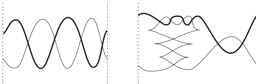
Figure 1.5: Minimal legendrian links 4 and (4, 3, 2) = \frac{30}{13}
