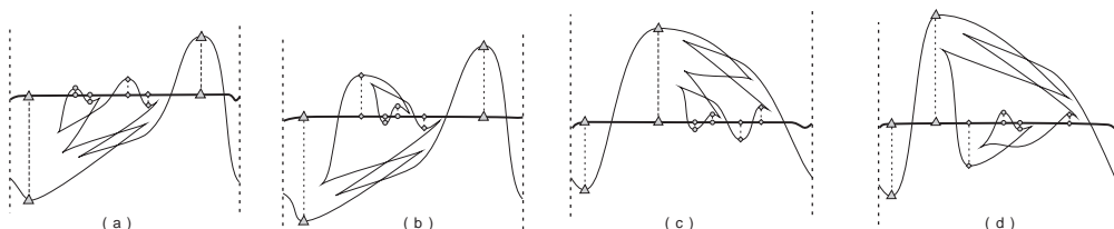
Figure 6.2.1: Links that differ by horizontal flypes: (a) (2, 1, 2, 2, 2) , (b) (2, 1, 2^1, 2, 2) , (c) (2, 1, 2, 2, 2^1) , (d) (2, 1, 2^1, 2, 2^1) . If L and L' differ by a horizontal flype from the j^{th} component, then there will be a change in the indices of the critical points associated to the terms h_{j+1}, \dots, h_n .
