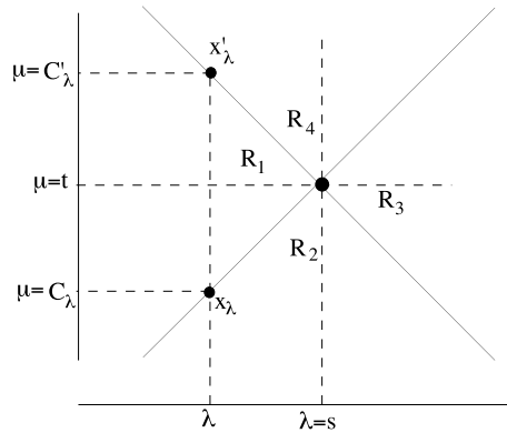
Figure 8: Configuration of (s; t) in
