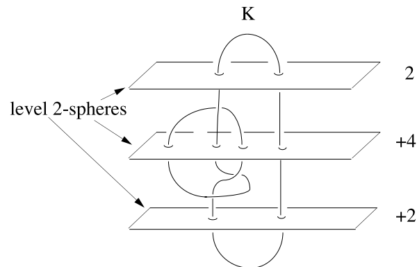
Figure 1: Thin presentation of complexity 8
