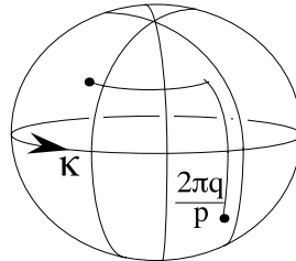
Figure 2: Standard spine of L(p; q) and core
