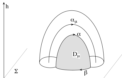
Figure 6: Inessential local maximum
