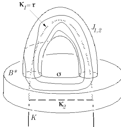
Figure 11: Standard spine in Z
