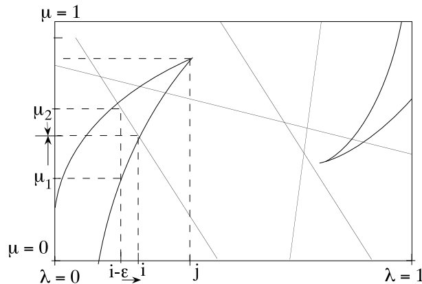
Figure 7: Graph of singularities
