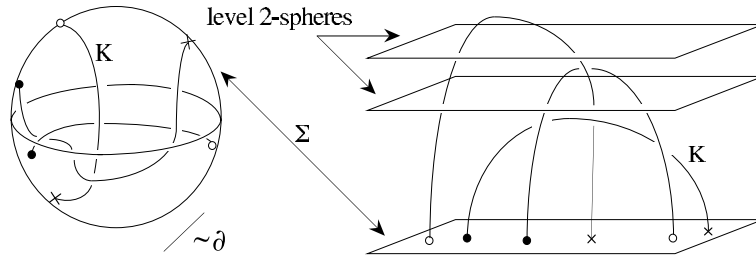
Figure 3: Morse presentation in a 3-manifold
