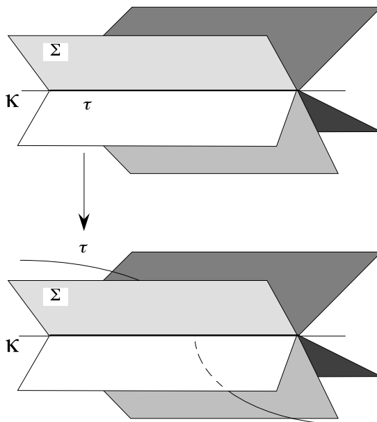
Figure 12: Isotopy of K with respect to the spinal helix
