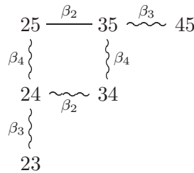
Figure 8: \mathcal{C}(\rho_{23}^6) with a maximal tree
