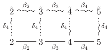
Figure 9: \mathcal{C}(\rho_4^6) with a maximal tree
