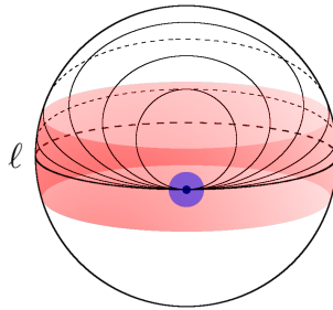
Figure 19: By a thin homotopy, the region around the equator is made to sit at the loop \ell around the equator so that the nearby loops drawn in the shaded region agree with \ell . The family of all these loops define a marking.
