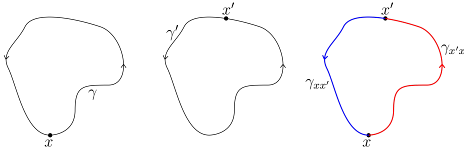
Figure 9: For two markings with associated basepoints x and x' of a thin loop [\gamma] , there exist representatives paths with sitting instants (shown on the right) \gamma_{x'x} : x \rightarrow x' (in red) and \gamma_{xx'} : x' \rightarrow x (in blue) such that \gamma := \gamma_{xx'} \circ \gamma_{x'x} (shown on the left) represents one marking and \gamma' := \gamma_{x'x} \circ \gamma_{xx'} (shown in the middle) represents the other. Note that \gamma' and \overline{\gamma_{xx'}} \circ \gamma \circ \gamma_{xx'} are thinly homotopic.
