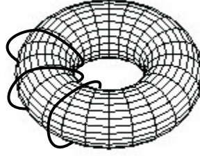
Figure 4. Wrapping of a string on an internal torus.
