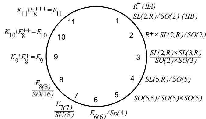
Figure 9. M(oduli)-theory clock.
