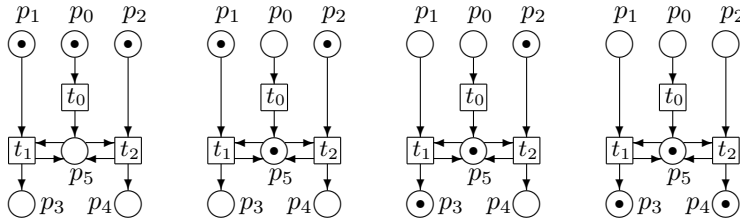
Figure 3: The behaviour of a Petri net.
