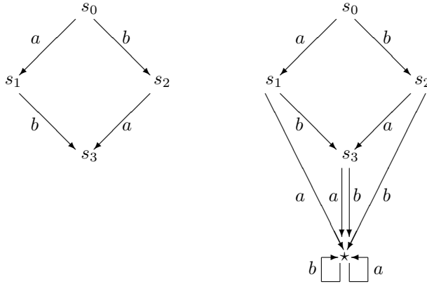
Figure 4: The graph and augmented graph of states
