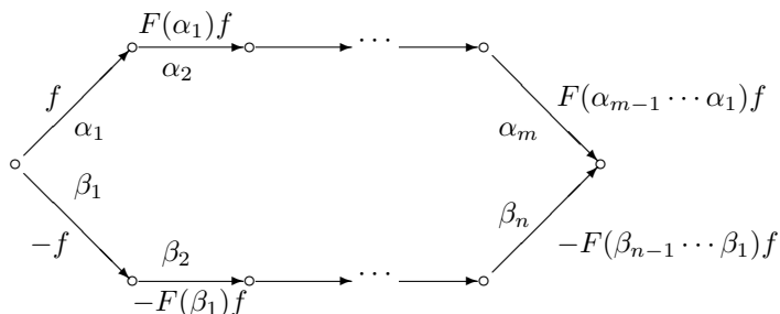
Figure 2: The internal flow d_1(f[r])
