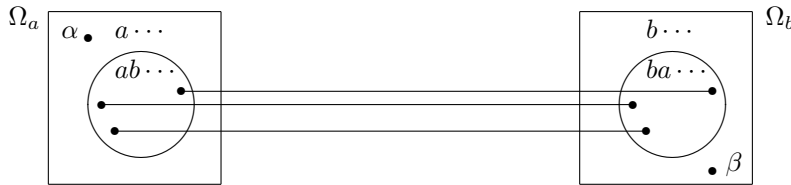
Figure 1: A graph containing the 2-paths \alpha \rightarrow \beta
