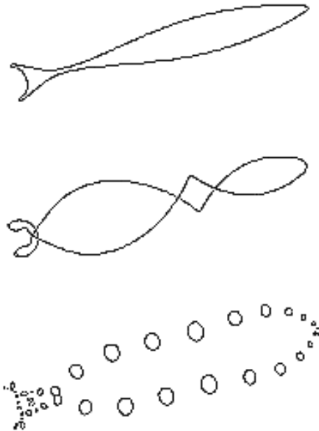
FIGURE 14. Bifurcation of one coset orbit.
