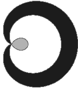
FIGURE 4. The set Q_2 .
